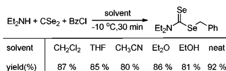
Scheme 3. Screening of Solvents
